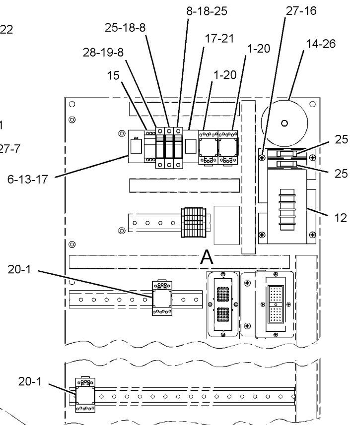
FRONT VIEW (ELECTRONIC PANEL)
