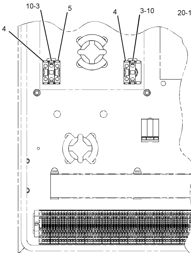
REAR VIEW (CONTROL PANEL)
